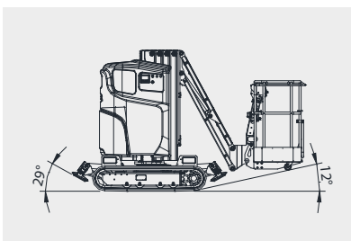
Jib free when machine stowed
