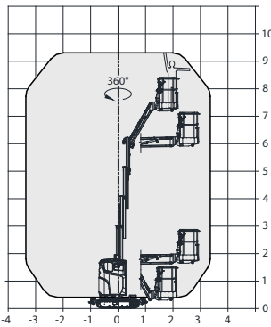
Working diagram on crawlers
