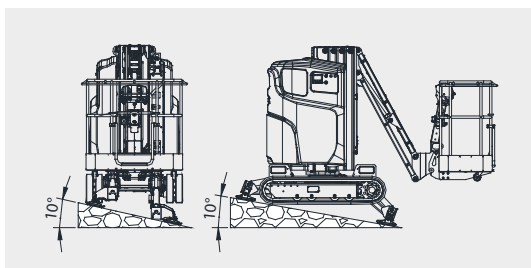
Max. tilt for selfstabilizers
