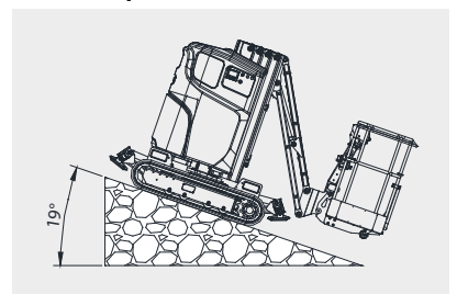
Max. slope 35%
